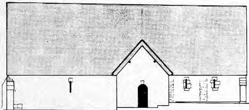
4. WEST ELEVATION
